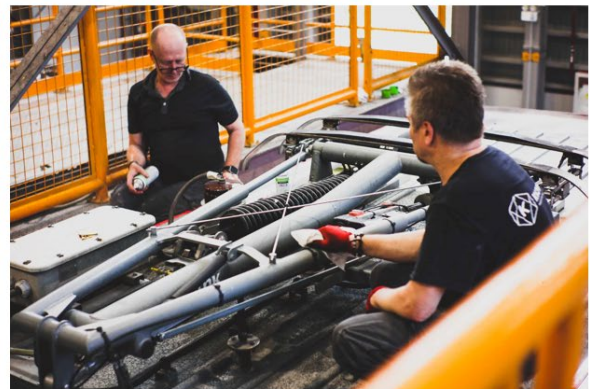
15 December 2023: Non-Destructive Testing of G4 Trainset 14 in Baclaran Expansion Depot, Pasay City.
